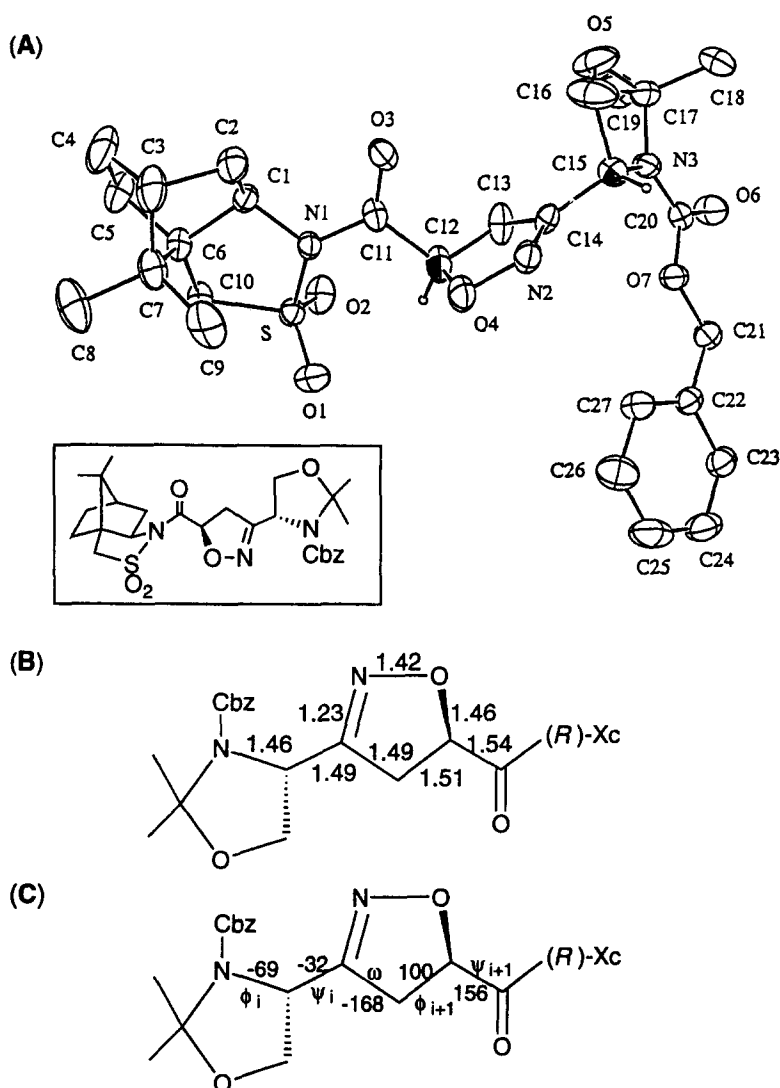
Figure 2. X-ray crystal structure (A) of cycloadduct 23 , bond length (Å, B), and torsion angle (deg, C) at the dipeptide unit for 23 .
