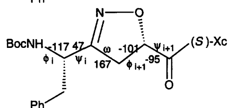
Figure 1. X-ray crystal structure (A) of cycloadduct 20 , bond length (Å, B), and torsion angle (deg, C) in the dipeptide unit for 20 .
