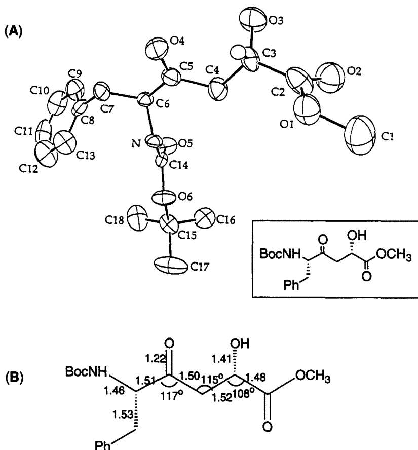
Figure 3. X-ray crystal structure (A), bond length (Å) and bond angle (deg, B) for the compound 41.
